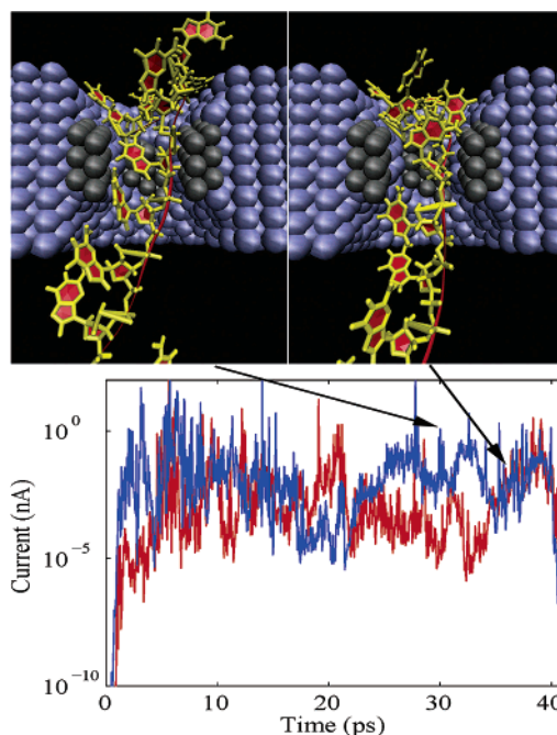
Figure 2. Current as a function of time for a poly(dC) 15 translocating through a nanopore. Blue (red) curve indicates the current, for a bias of 1 V, between the right and left (front and back) electrodes represented in gray in the snapshots (the fourth electrode is located behind the field of view and is hence not visible in the snapshots). During approximately the first half of the translocation, the two currents follow each other, indicating that no bases are aligned with either electrode pair. The left snapshot indicates the case in which a nucleotide is aligned with a pair of electrodes; the right snapshot when the nucleotide is not aligned between either pair of electrodes. In the snapshots, solution atoms are not shown and red colors are a guide for the eye only.
